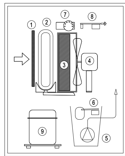
Fig. 3 Machines with condensed water lifting pump
