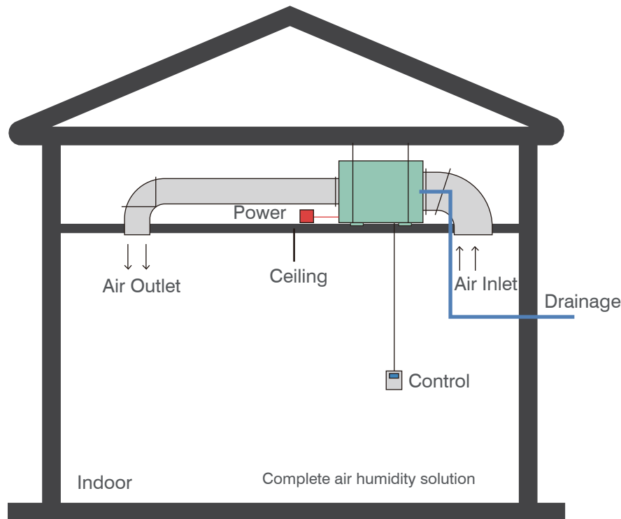
Ceiling Dehumidifier Working Principle
